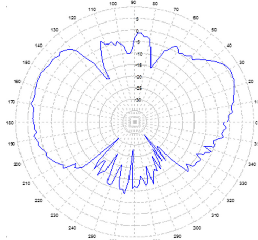
5.85 GHz. AZIMUTH
