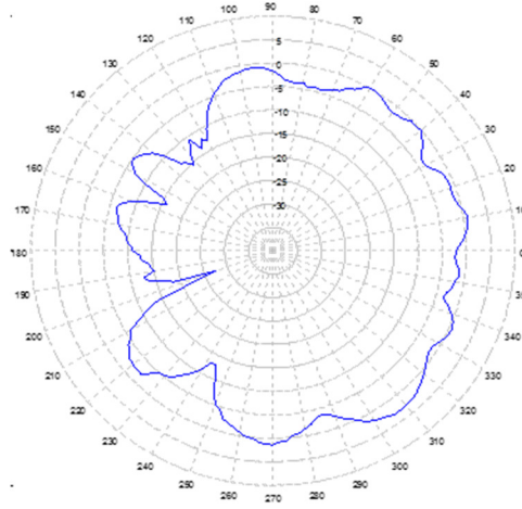
4.95 GHz. AZIMUTH
