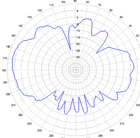
5.35 GHz. AZIMUTH
